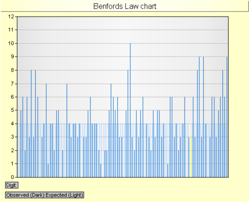
Example Chart - Test of Last Two Digits (L2)
