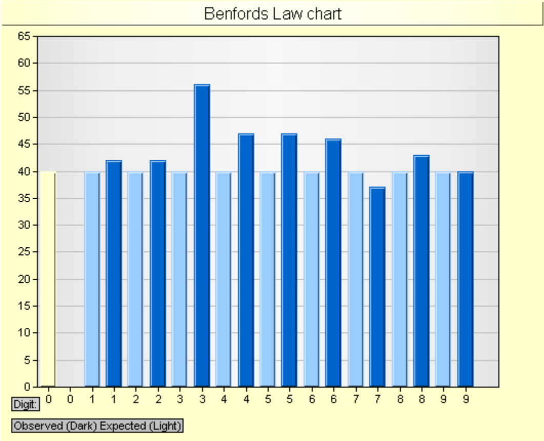
Example Chart - Test of Last Digit (L1)
