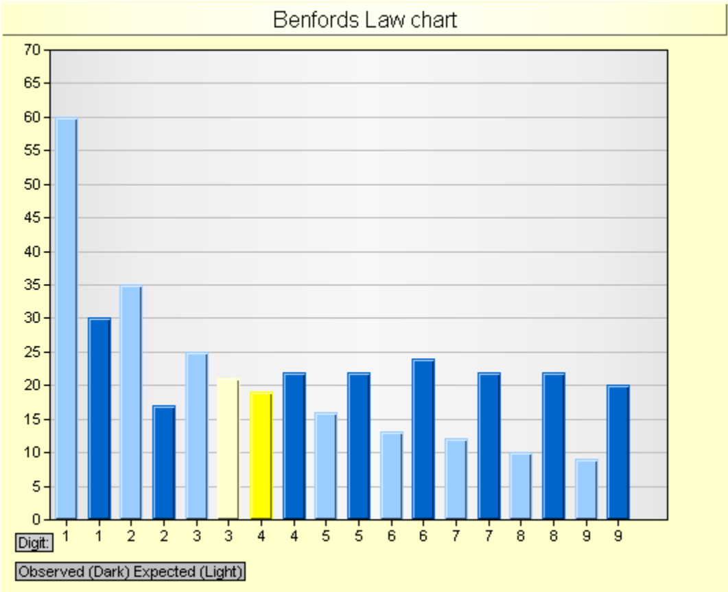
Example Chart - Test of First Digit (F1)
